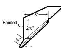
LG 120 DENVER EAVE TRIM
