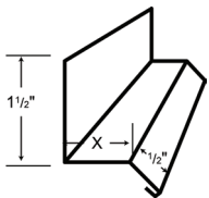
LG 138 / LG 139 "W" FORMED VALLEY*
