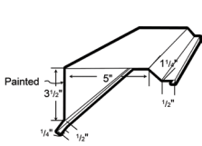
LG 118 DENVER GABLE
